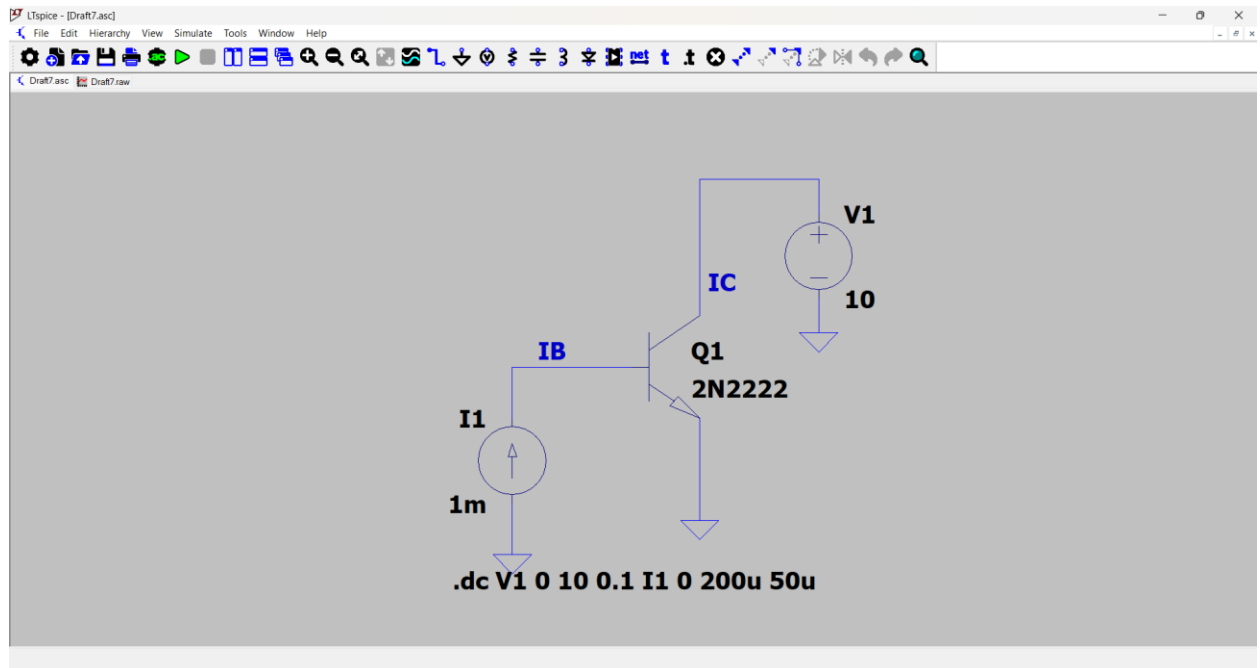
Screenshot 5 : Schematic Diagram
